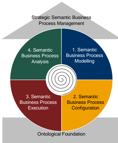
Fig. 1. Semantic BPM life cycle, adapted from [7].
